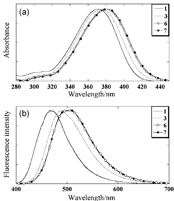
Fig. 1. (a) UV-vis absorption spectra for 1 , 3 , caged glutamate 6 , and caged GABA 7 in HEPES buffer at pH 7.2.
