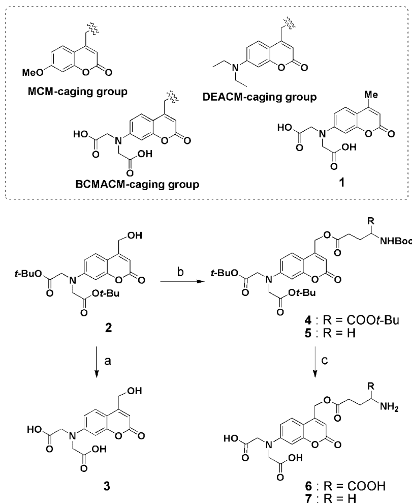
Scheme 1. (a) TFA, CH 2 Cl 2 , H 2 O, rt, 20 min; (b) EDC, DMAP, CH 2 Cl 2 , N -Boc-Glu- O - t -Bu for 4 , or N -Boc-GABA for 5 , rt, 40 min.
