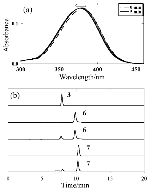
Fig. 2. (a) Change in the absorption spectra of 6 in HEPES buffer ( 1.0 \times 10^{-5} M) at pH 7.2 on photoirradiation with 380 nm light. (b) HPLC chromatograms of 3 as an authentic sample, 6 before irradiation, 6 after irradiation, 7 before irradiation, and 7 after irradiation from the top to the bottom, respectively.
